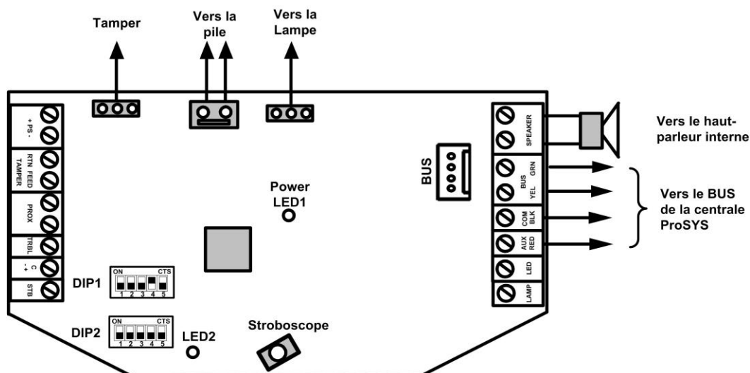
Figure 2 - Configuration BUS
